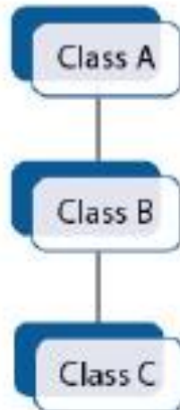
Multilevel Inheritance
