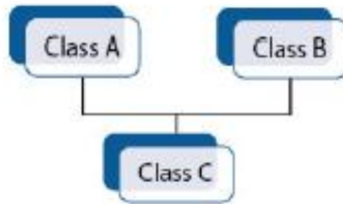
Multiple Inheritance
