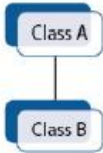
Single Inheritance
