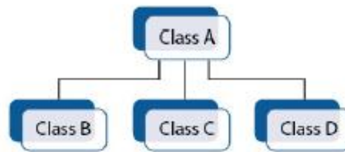
Hierarchical Inheritance
