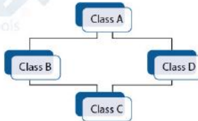
Hybrid Inheritance
